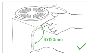
During normal service, once need a turning, must hold the curve of LED strip with its front side up and back side down. (Attention: keep the curved radian \geq 120\text{mm} )
